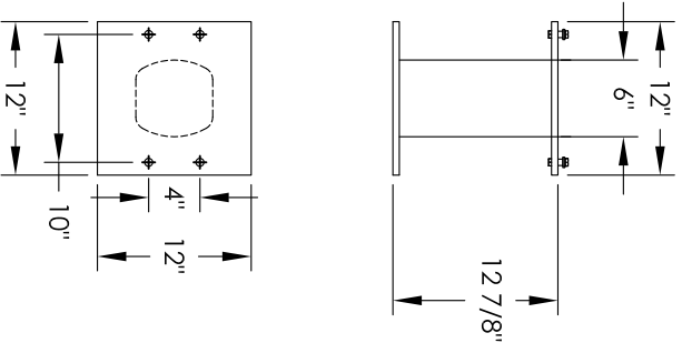
PEDESTAL DETAIL
