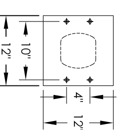
PEDESTAL DETAIL
